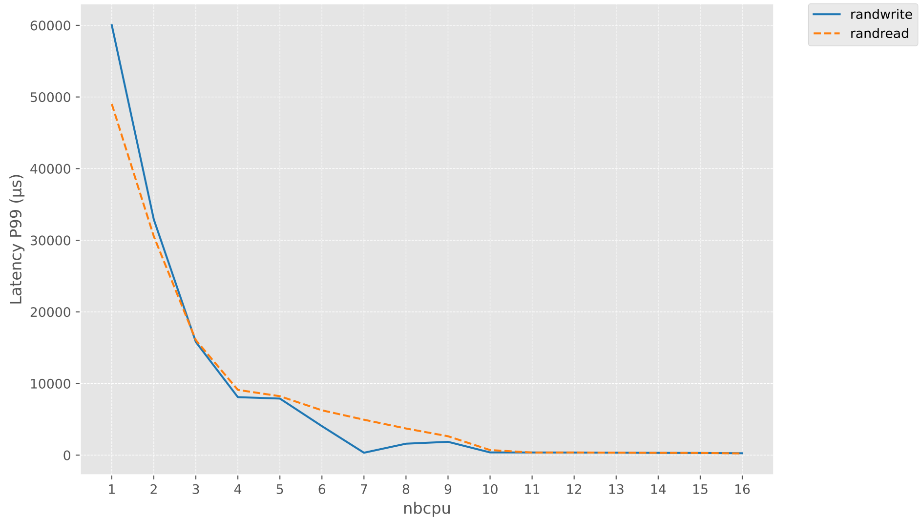
Latency P99 vs nbcpu
